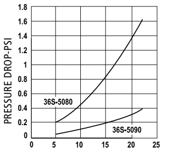
FLOW RATE-GPM (STODDARD SOLVENT)
